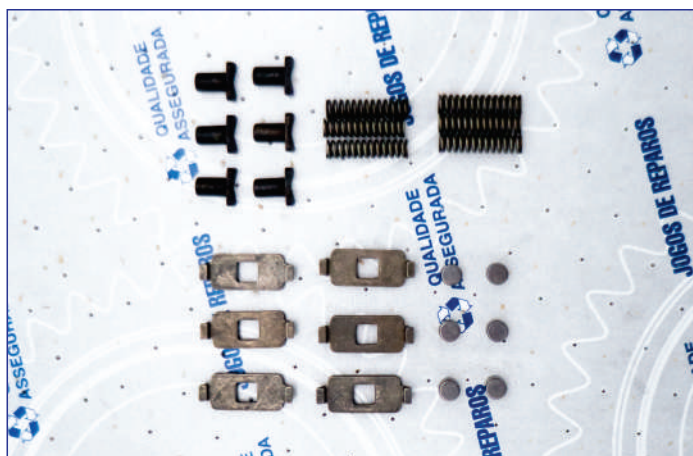
30894 – JOGO DE PRESSIONADOR DA REDUZIDA R/SR 1400/1700, R/SR 1900/2000, SRO 2000/2400 (1653904x6, 1653901x6, 1668280x6, 1653991x6)
