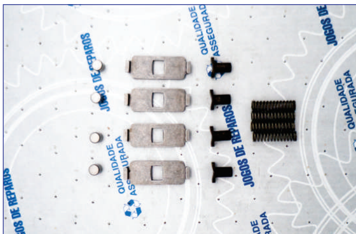
30890 – JOGO DE PRESSIONADOR DAS MARCHAS R/SR 1400/1700, R/SR 1900/2000, SRO 2000/2400 (1653900X4, 1653901X4, 1653994X4, 1668280X4)
