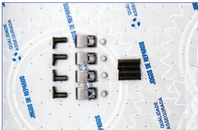
30891 – JOGO DE PRESSIONADOR DAS MARCHAS R/SR 1400/1700, R/SR 1900/2000, SRO 2000/2400 (1653900X4, 1653901X4, 1653983X4, 1653995X4)
